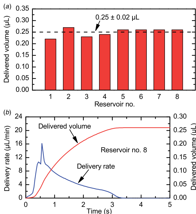
Figure 9. Representative delivery characteristic of a micropump after individual heating with 225 mW for 10 s. (a) Delivered liquid volumes in consecutive order for one half of the device. (b) Transient delivery rate and delivered volume for reservoir no. 8.
