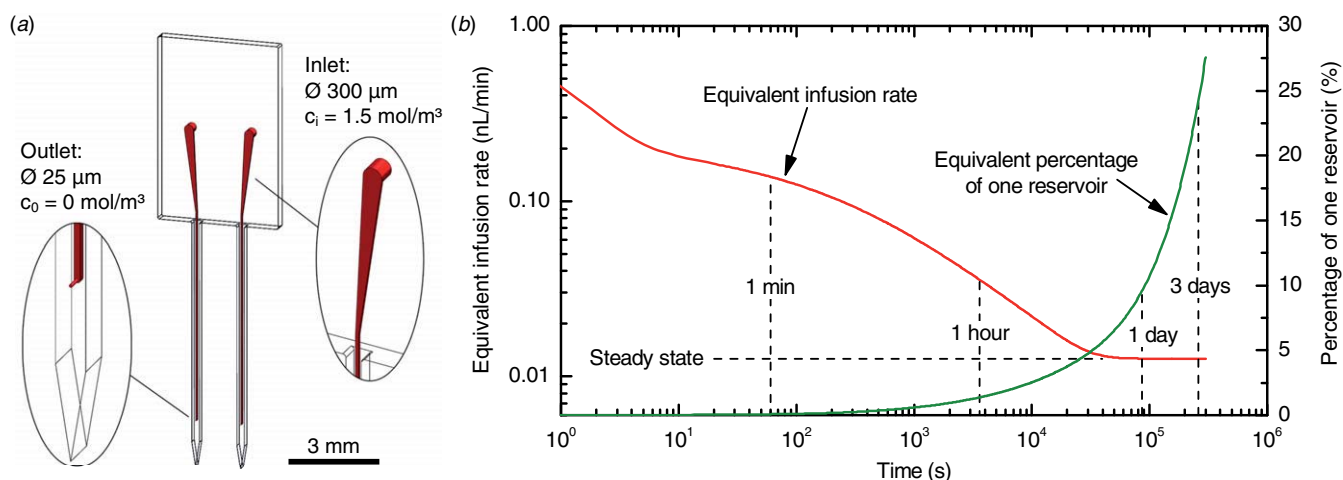
Figure 2. CFD-simulation of the diffusion-based leakage from the probe outlet. (a) Microprobe geometry. (b) Leakage rate expressed as an equivalent infusion rate and total drug amount lost over time expressed as percentage of the amount stored in a 0.25 \mu\text{L} reservoir.
