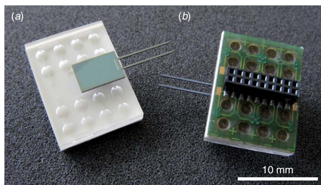
Figure 8. Assembled NeuroMedicators showing (a) the top side with the liquid reservoirs and the microprobes as well as (b) the bottom side with the electrical micro connector.
